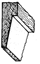
Ship Lap
